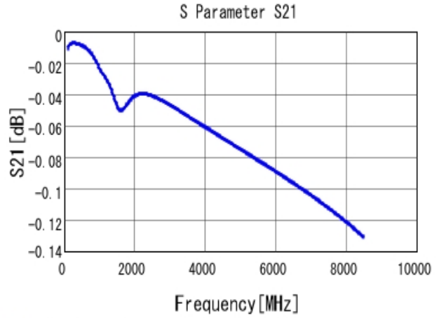
■ GRM0335C1E471JA01 S21 DCOV, 25degC
