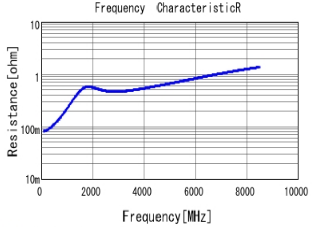
■ GRM0335C1E391GA01 R DC0V, 25degC
