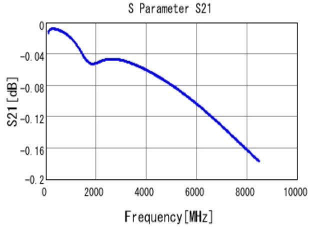
■ GRM0335C1E391GA01 S21 DCOV, 25degC
