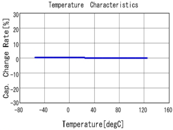
■ GRM0335C1E391GA01 C-Temp. capchange, DCOV, AC1Vrms
