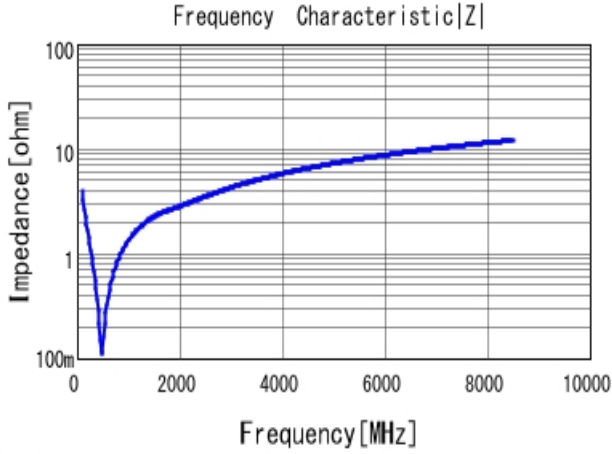
■ GRM0335C1E391GA01 |Z| DC0V, 25degC
