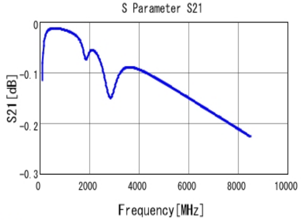
■ GCM1555G1H101JA16 S21 DCOV, 25degC
