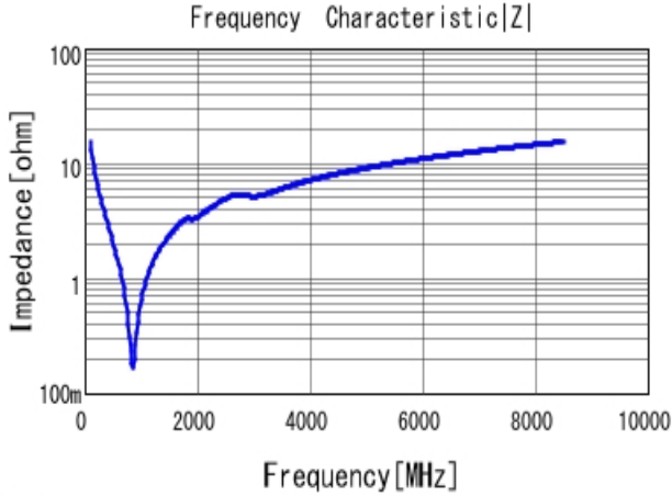
■ GCM1555G1H101JA16 |Z| DC0V, 25degC
