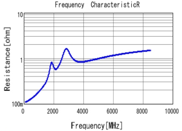
■ GCM1555G1H101JA16 R DC0V, 25degC
