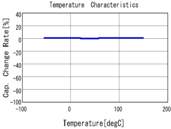
■ GCM1555G1H101JA16 C-Temp. capchange, DCOV, AC1Vrms
