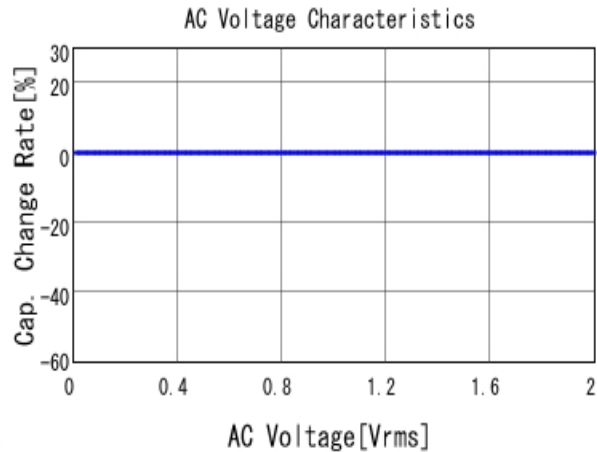
■ GCM1555G1H101JA16 C-AC Voltage capchange, DC0V, 25.0d
