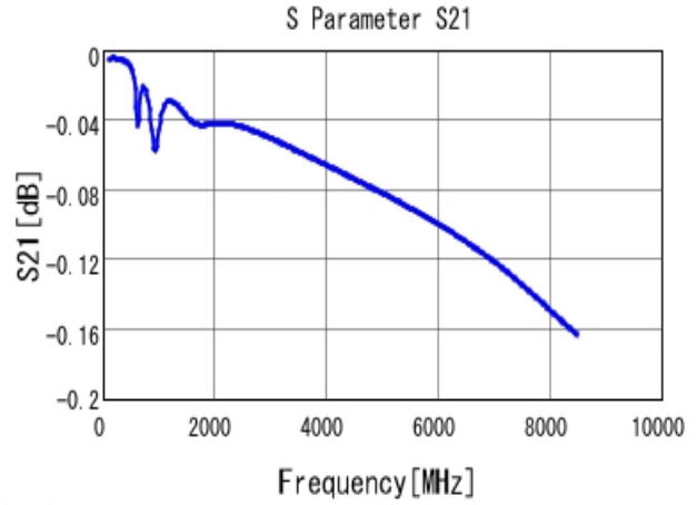
■ GCM1555C1H821JA16 S21 DCOV, 25degC
