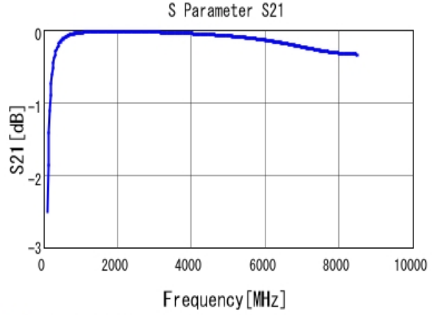
■ GCM0335C1H180FA16 S21 DCOV, 25degC
