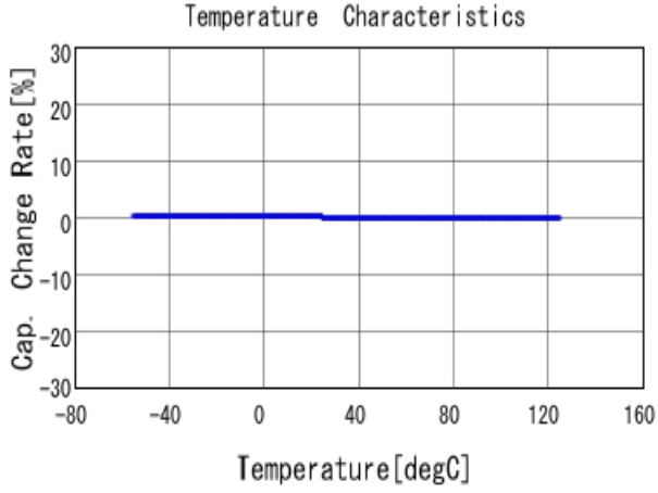
■ GCM0335C1H180FA16 C-Temp. capchange, DCOV, AC1Vrms
