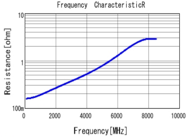
GCM0335C1H180FA16 R DC0V, 25degC
