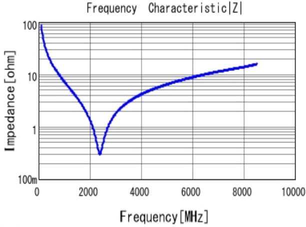
GCM0335C1H180FA16 |Z| DC0V, 25degC
