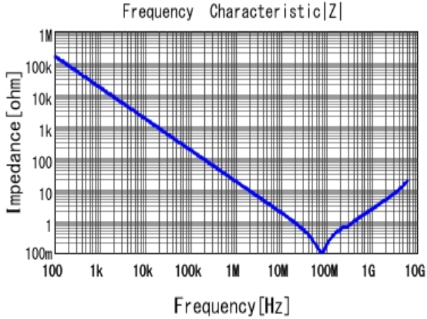
■ GCJ188R91H103KA01 |Z| DCOV, 25degC
