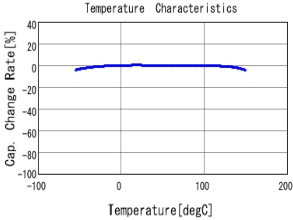
■ GCJ188R91H103KA01 C-Temp. capchange, DC0.0V, AC1.0V rm
