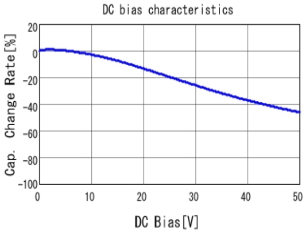
■ GCJ188R91H103KA01 C-DC bias capchange, 25.0degC, AC1.
