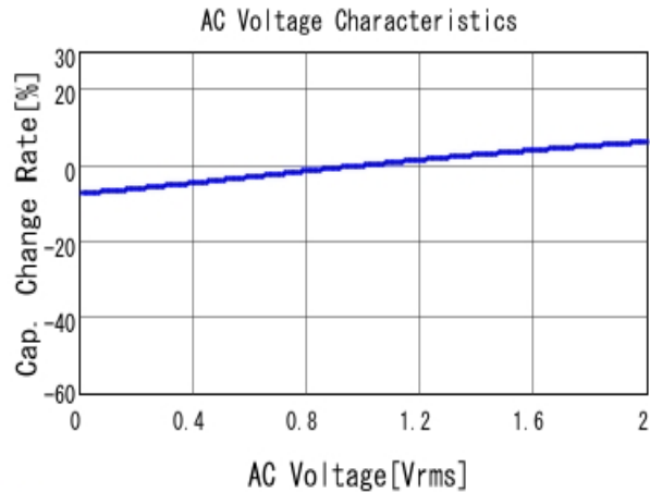
■ GCJ188R91H103KA01 C-AC Voltage capchange, DCOV, 25.0d
