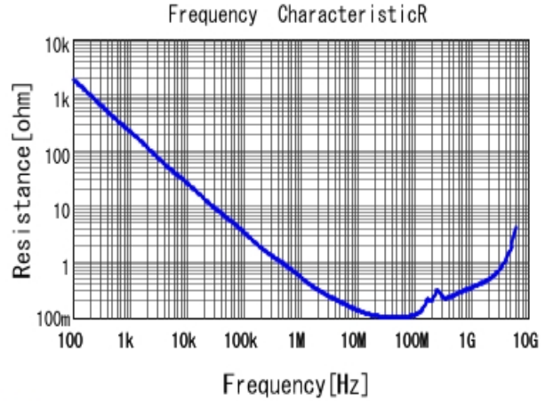
■ GCJ188R91H103KA01 R DCOV, 25degC
