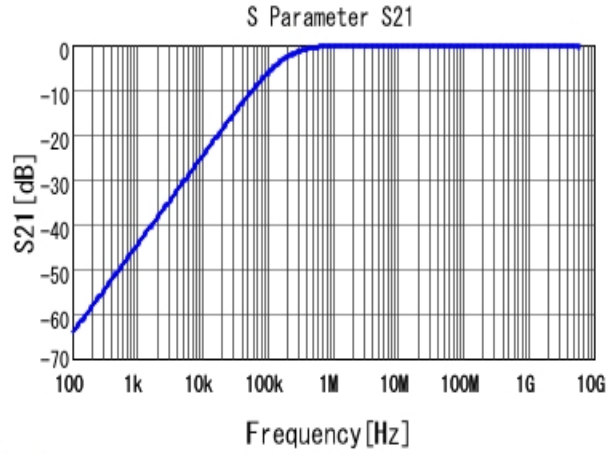
■ GCJ188R91H103KA01 S21 DC0V, 25degC
