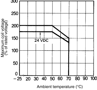
Ambient Temperature vs. Maximum Voltage (reference only)
