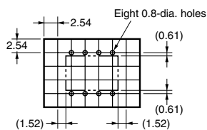
G3VM-352C
