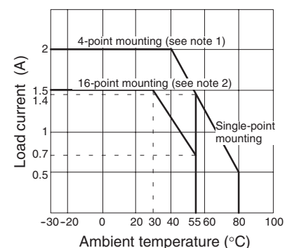
G3R-OA202SZN/OA202SLN
