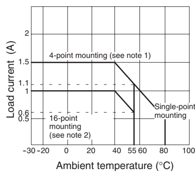
G3R-OD201SN (40 to 200 VAC)
