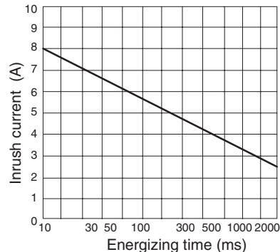
G3R-OD201SN
