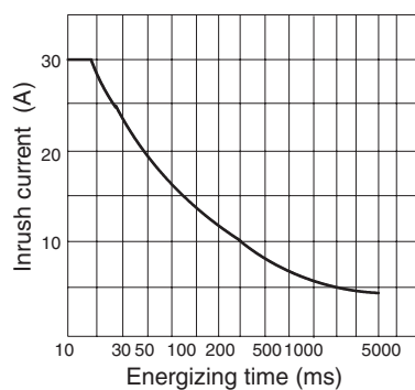
G3R-OA202SZN/OA202SLN
