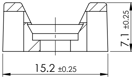
SECTION X-X
