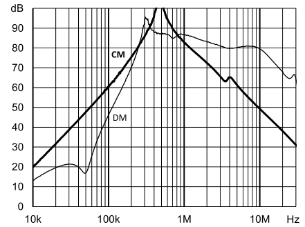
FN 3288-50-53-C35-R65
