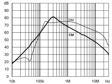
FN 3288-100-35-C35-R65
