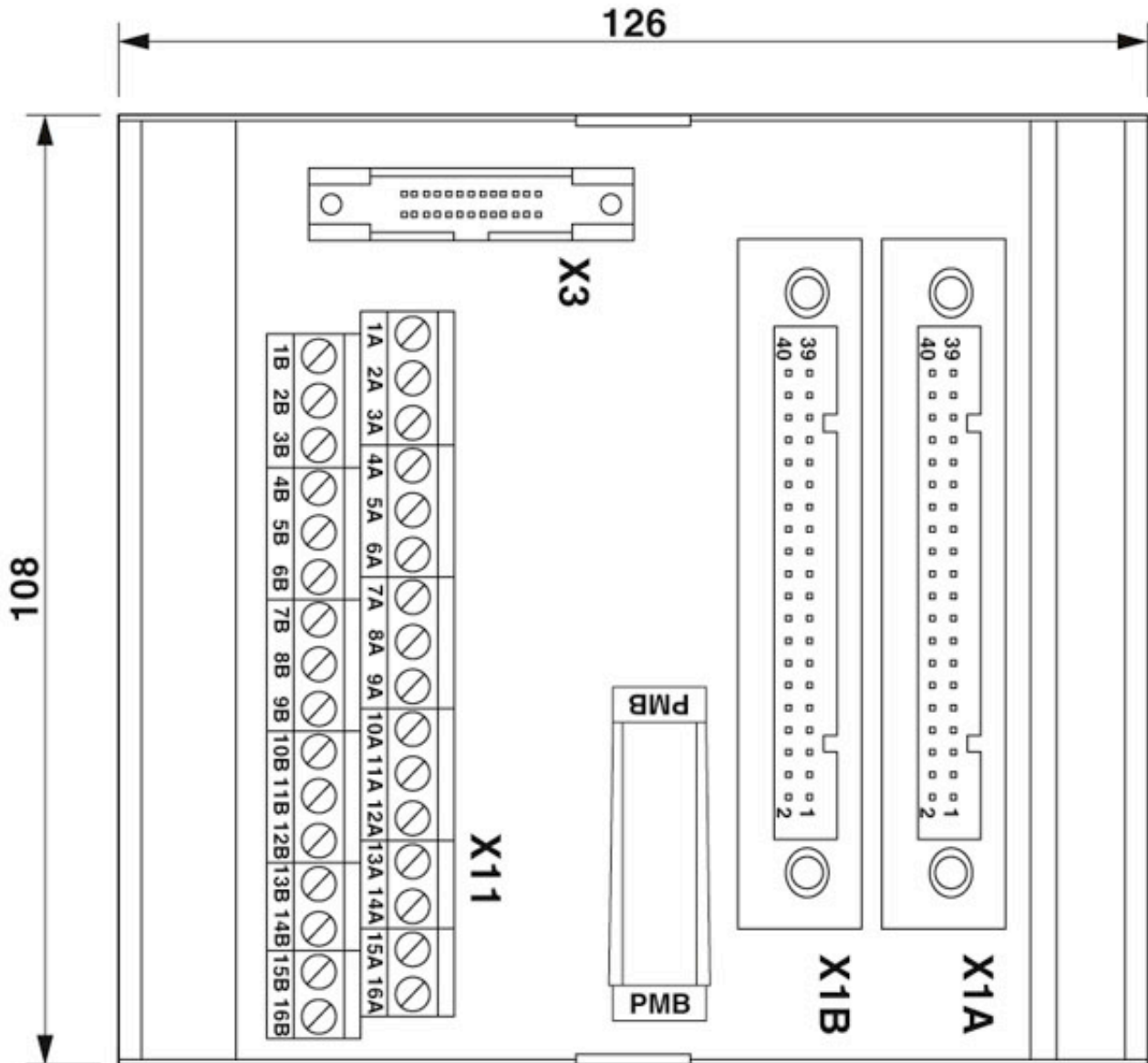
Dimensional drawing
