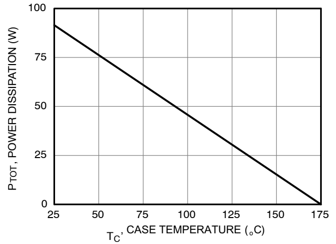
Figure 4. Power Derating
