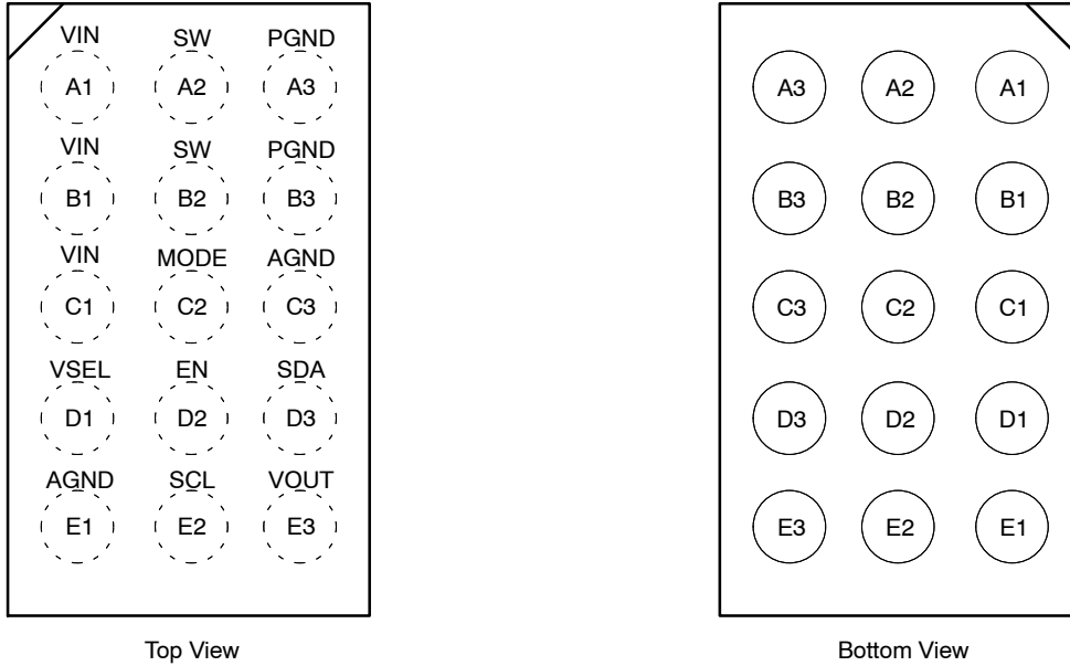
Figure 2. Pin Configuration
