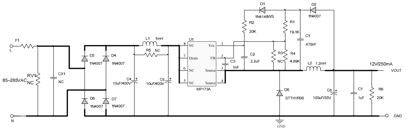
Figure 1: Schematic
