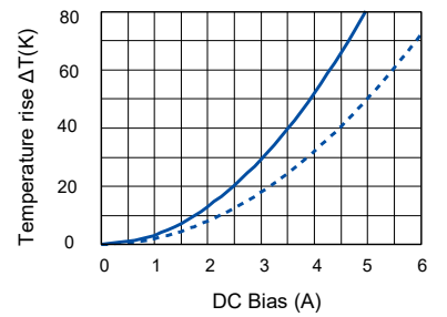
[ ETQP4M100YFN ]
