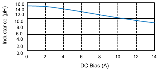
[ ETQP6M150KLC ]
