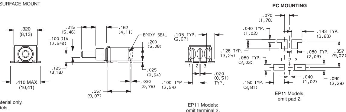
EP12SD1SAPE SPDT
