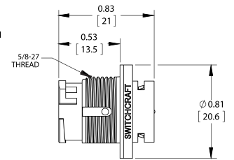
OPTION "C" EN3 SERIES 9-18 POSITION CRIMP TERMINALS EN3P2MCX SHOWN
