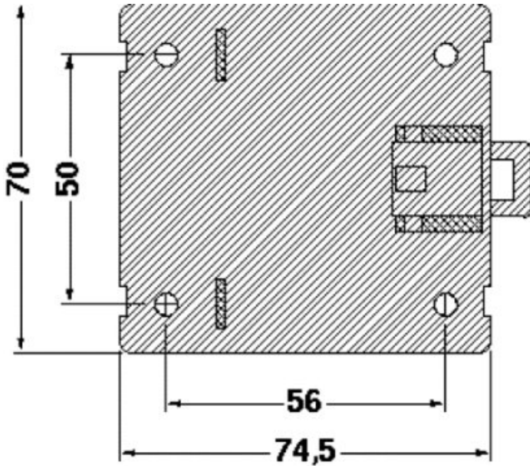
Dimensional drawing
