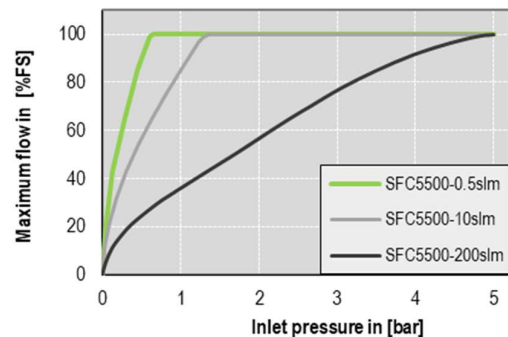
Figure 8 Maximum achievable flow rate at different input pressures.
