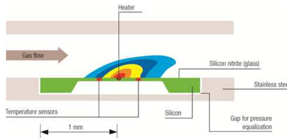
Figure 3: Cross-sectional view of gas channel.
