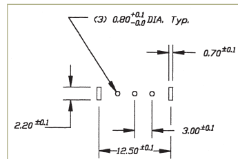
P.C. MOUNTING
