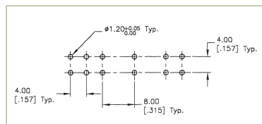
P.C. MOUNTING
