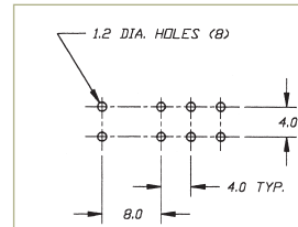
P.C. MOUNTING
