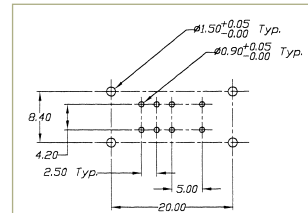
P.C. MOUNTING
