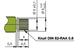
TYPE 44 - BRASS
