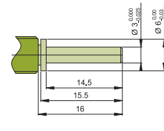
TYPE 40 - BRASS
