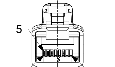
PIN 1 CONNECTOR PIN ASSIGNMENT VIEW FROM THE FRONT SIDE M12 HIED FOR CLARITY SCALE 2:1
