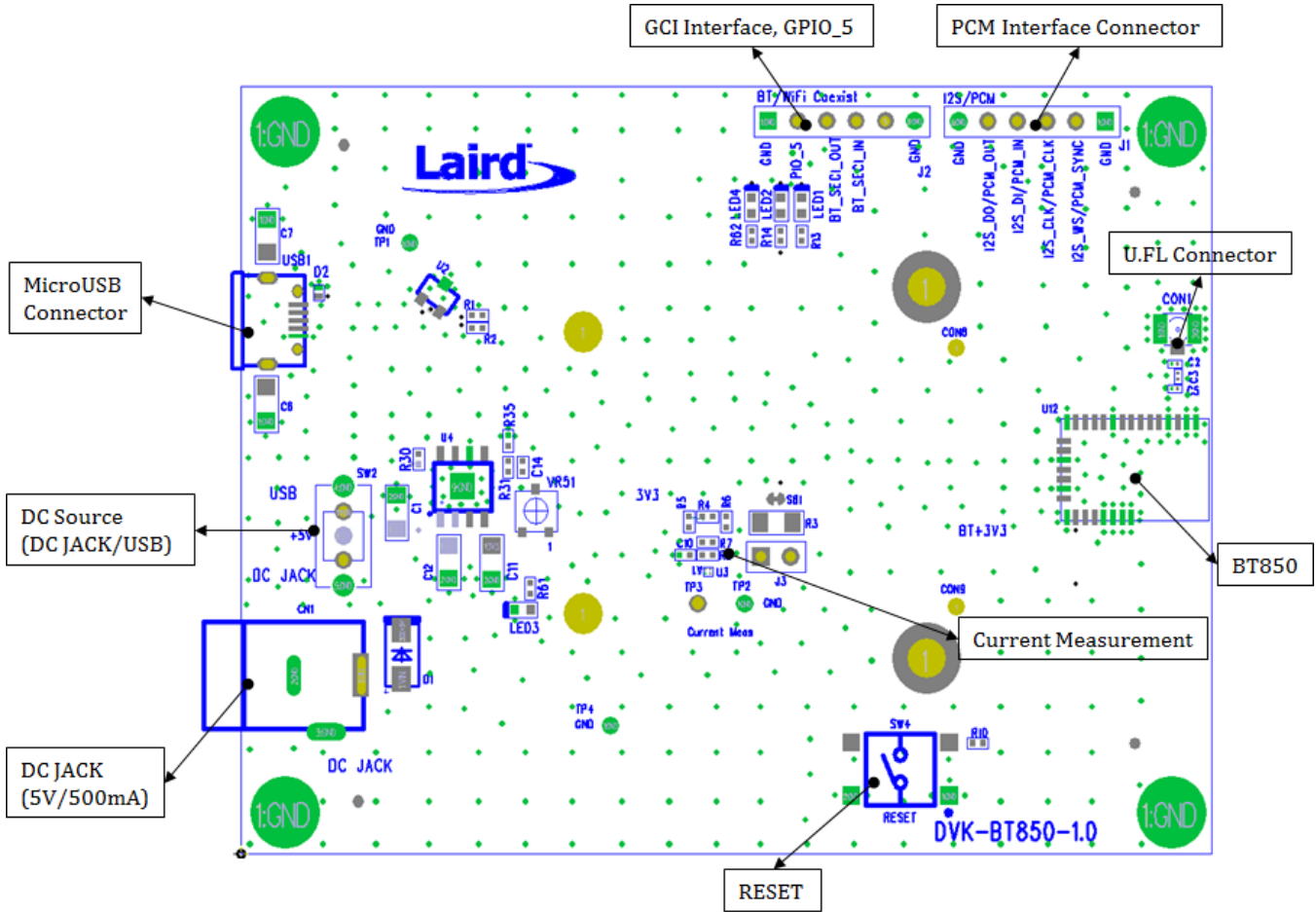
Figure 1: Main DVK-BT850-Sx Board
