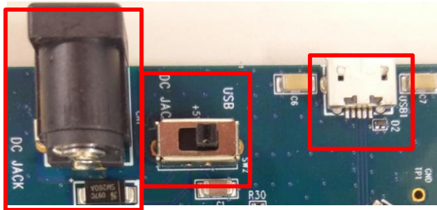
Figure 6: Micro-USB Connector (USB1), SW2, and DC JACCK (CN1)
