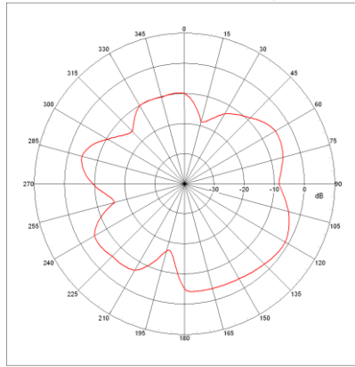
Far-field Power Distribution(H+V) on X-Z Plane Plot Peak Gain(H+V)=-1.3 dB, Plot AvgGain(H+V)=-7.4dB @2.44000 GHz
