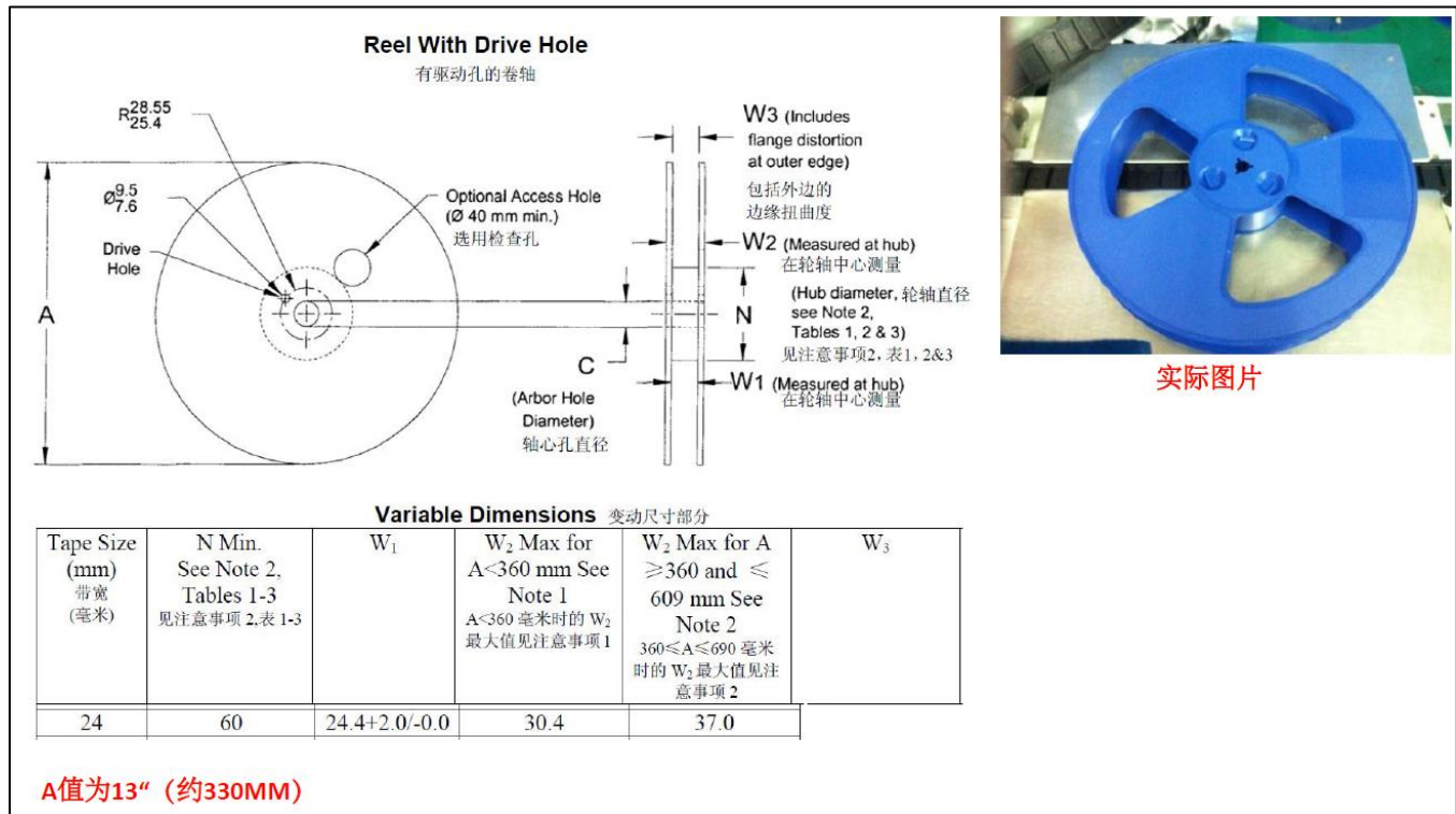
Figure 13: Reel specifications
