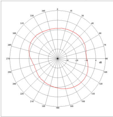
Far-field Power Distribution(H+V) on X-Y Plane Plot Peak Gain(H+V)=-5.1 dB, Plot AvgGain(H+V)=-8.7dB @2.44000 GHz
