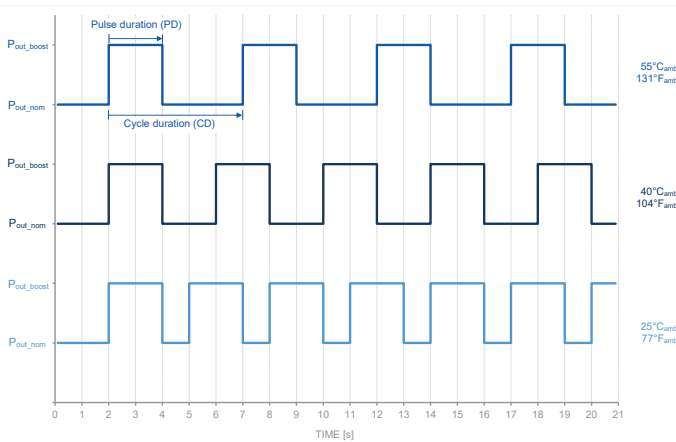
Fig. 10: Cycle duration in dependence of the ambient temperature and usage of the full boost power (120% / 2s)
