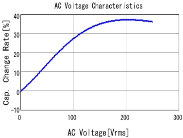
■ DE2E3SA102MN3AT02F C-AC Voltage capchange, DCOV, 20.0
