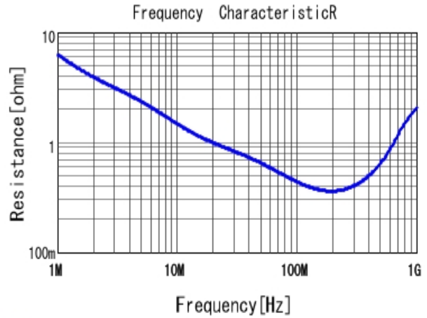
■ DE2E3SA102MN3AT02F R DCOV, 20degC
