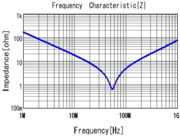
■ DE2E3SA102MN3AT02F |Z| DCOV, 20degC
