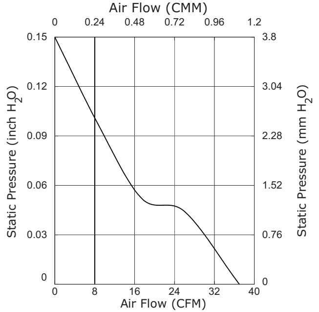
CFM-8025V-142-415
