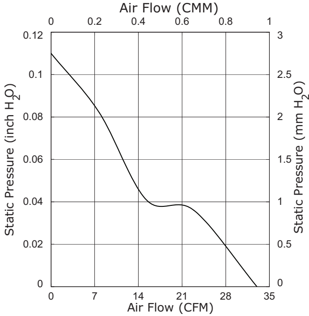
CFM-8025V-132-330
