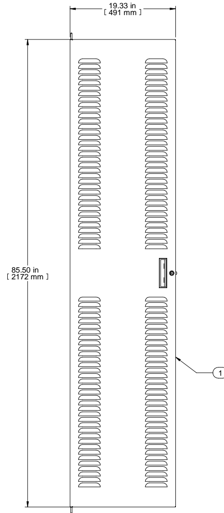
FRONT VIEW
