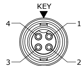
FACE VIEW P/N: CA63804PXXX90
