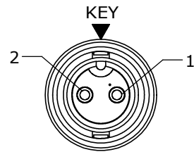
FACE VIEW P/N: CA63802PXXX90
