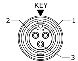
FACE VIEW P/N: CA63803PXXX90
