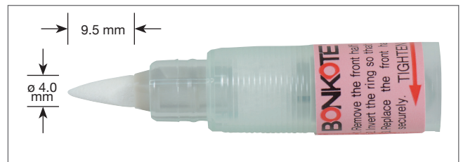
BR-102B Cap & Brush; Felt-type, thin
