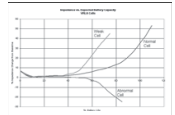
Figure 4. Impedance increases with battery age (and weakness)
