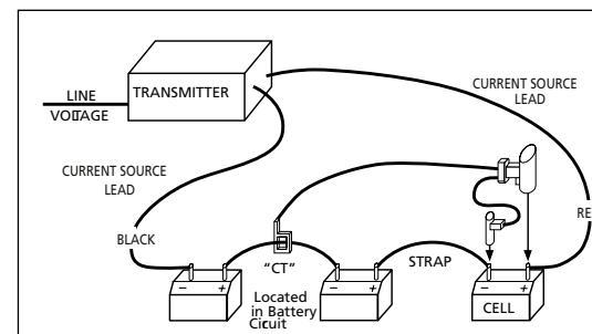
Figure 2. A typical test setup
