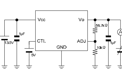
Measurement setup for Figure 15
