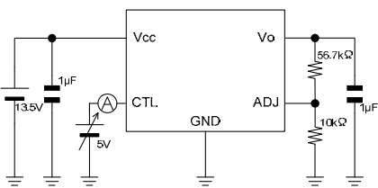
Measurement setup for Figure 20
