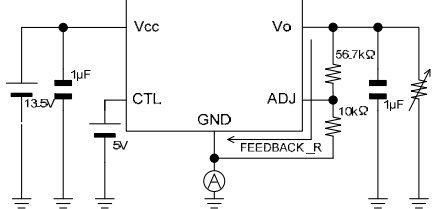
Measurement setup for Figure 19
