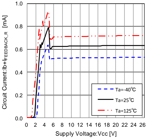
Figure 11. Circuit Current (IFEEDBACK_R(Note 1) ≈ 75μA)
