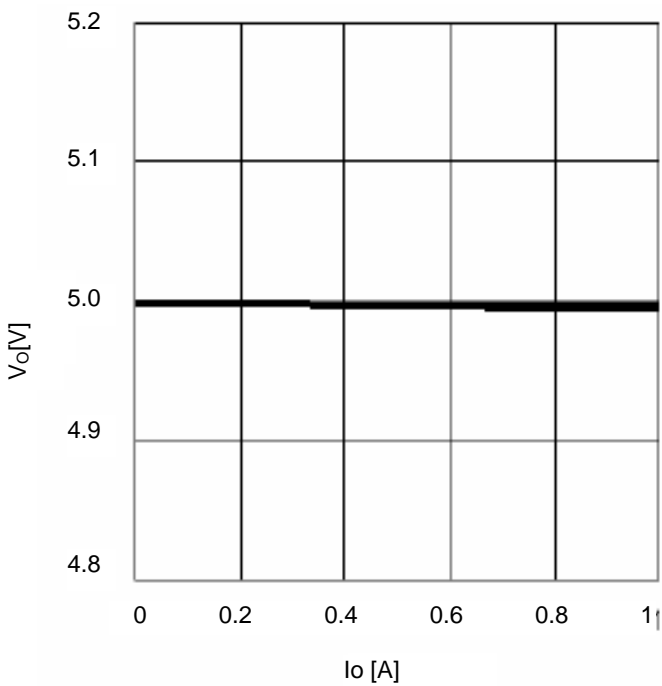
Figure 25. I_O - V_O
