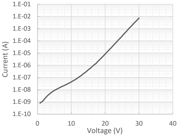
Current - Voltage
