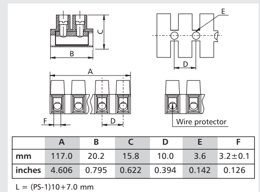
Dimensions in mm 1 mm = 0.0394 in.
