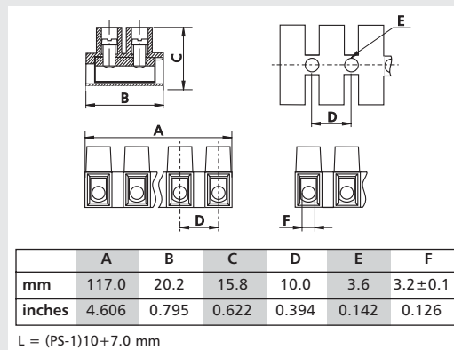
Dimensions in mm 1 mm = 0.0394 in.
