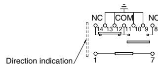
(Deenergized condition)
