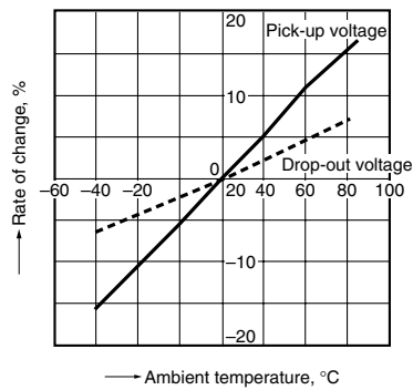
2. Ambient temperature characteristics Sample: 6 pcs., ALS2B12TW
