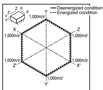
8. Malfunctional shock Tested sample: AGQ200A4H, 6 pcs.
