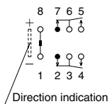
1 coil latching
