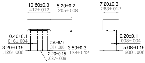
External dimensions
