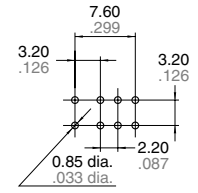
PC board pattern
