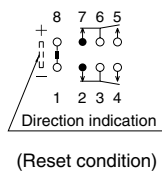
1 coil latching
