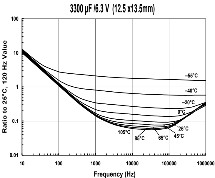
Impedance vs. Temperature and Frequency 3300 \mu F /6.3 V (12.5 x13.5mm)
