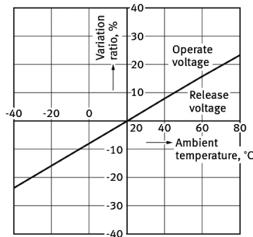
1-1. Ambient temperature characteristics (10A Type)
