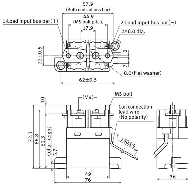
External dimensions
