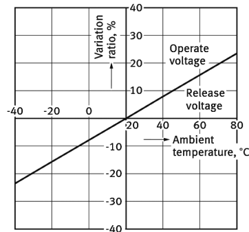
1-2. Ambient temperature characteristics (20A Type)
