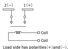
Schematic (TOP VIEW)
