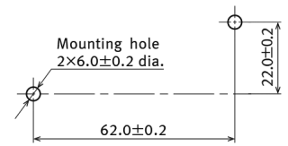
Mounting dimensions
