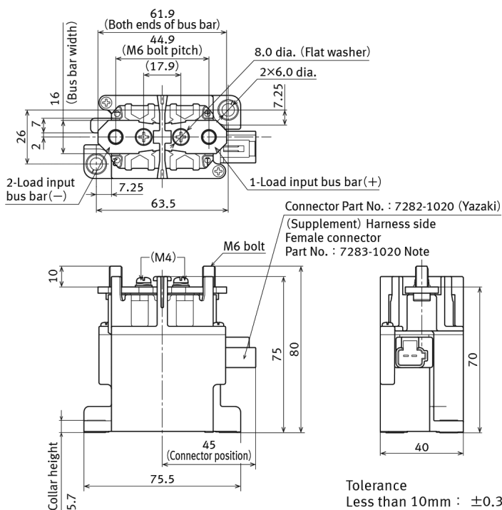
External dimensions
