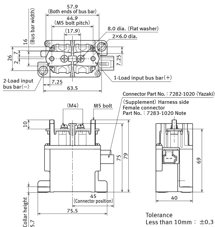
External dimensions
