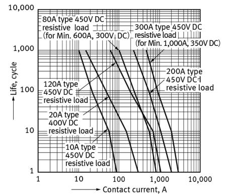
4. Switching and cut-off life curve (Forward direction)
