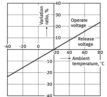
1-3. Ambient temperature characteristics (80A Type)
