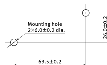
Mounting dimensions
