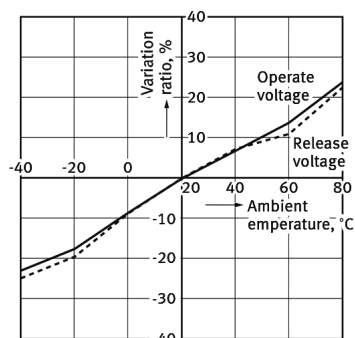
1. Ambient temperature characteristics
