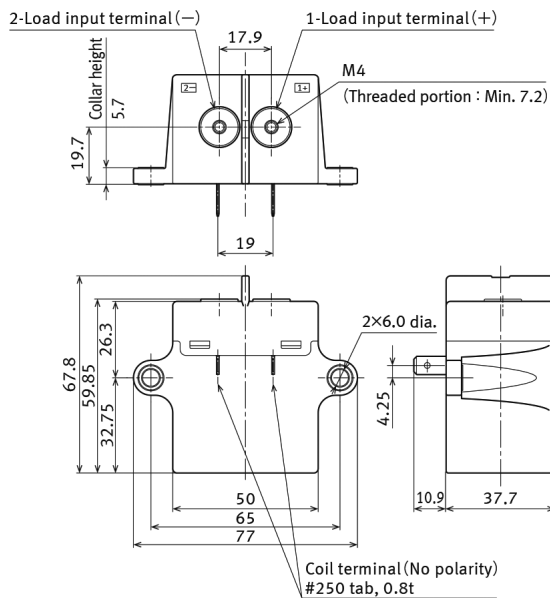
External dimensions
