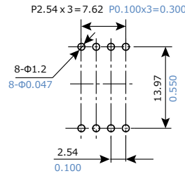
Recommended PC board pattern (TOP VIEW)
