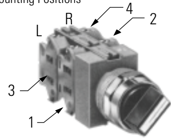
Mounting Positions
