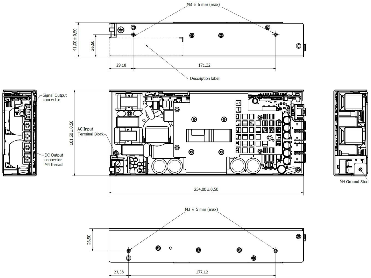
Figure 1. Mechanical Drawing - ABC1200-1T24-UCF Model
