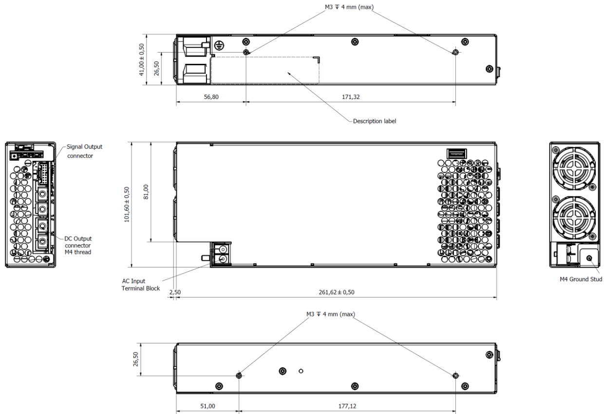
Figure 7. Mechanical Drawing - ABE1200-1T24 / ABE1200-1T48 Models
