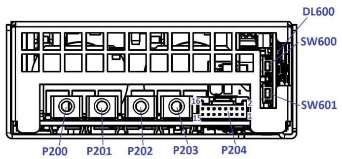
Figure 6. Rear View - ABC1200-1T24-PCF Model
