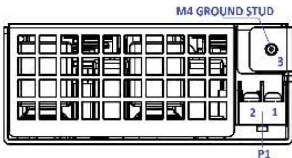
Figure 5. Front View - ABC1200-1T24-PCF Model
