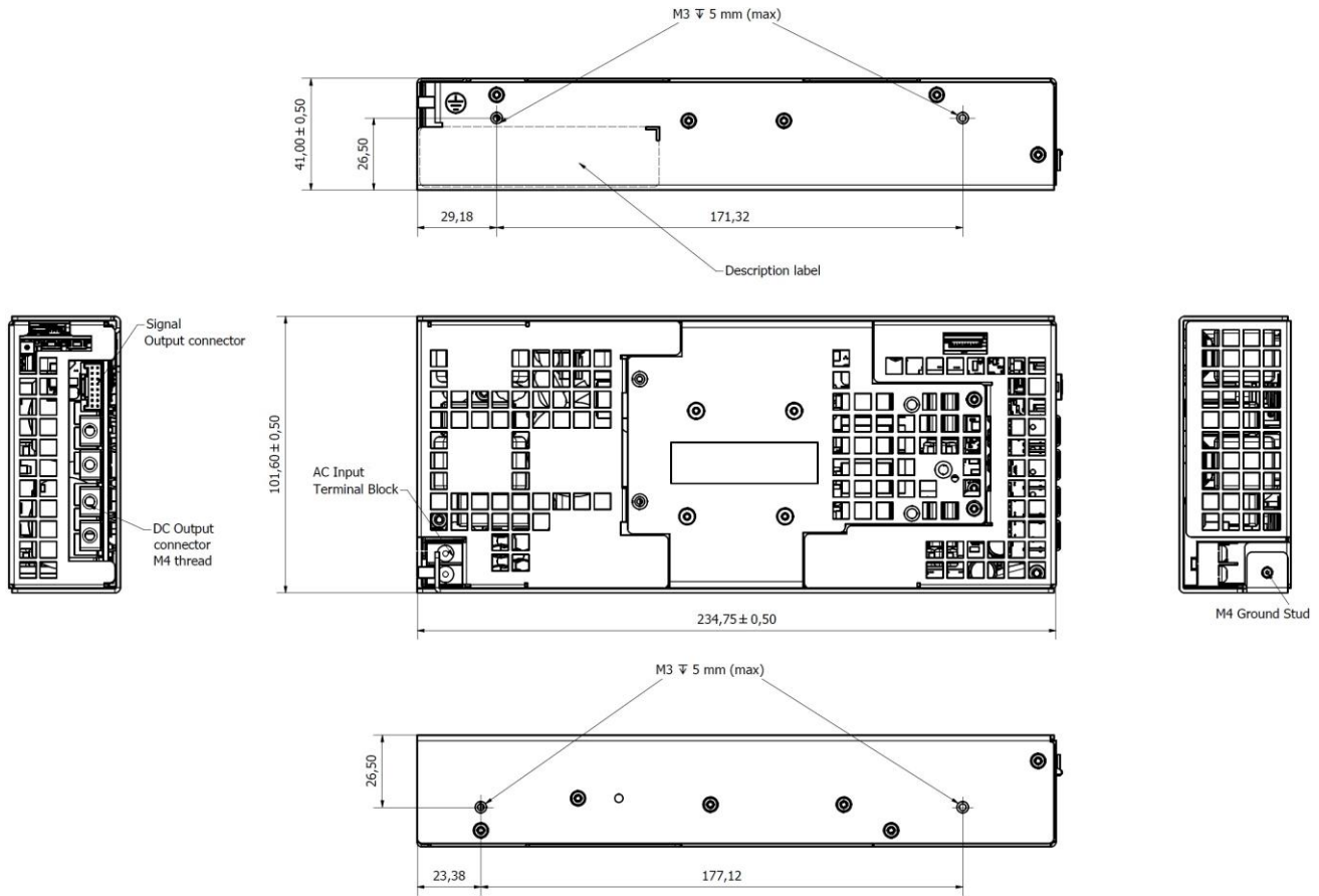
Figure 4. Mechanical Drawing - ABC1200-1T24-PCF Model
