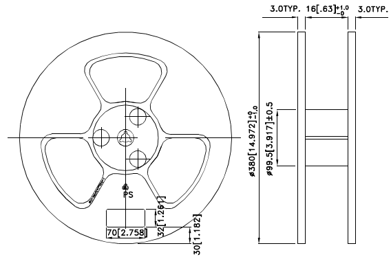
Reel Dimension
