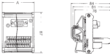
RSSD Poles/Dimensions
