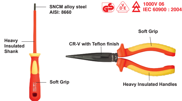
Screwdriver Specifications
