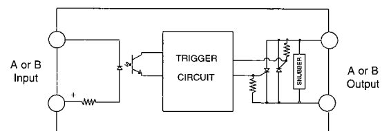
GD SERIES DC INPUT EQUIVALENT CIRCUIT
